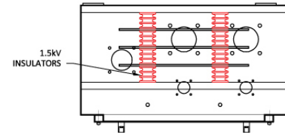
TOP SECTION-THROUGH
